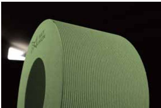
GFW for continuous generating grinding
